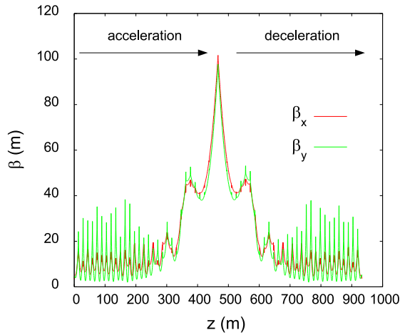
Figure 5: Optimum betatron envelopes obtained from the “minimum beam size” scheme.
