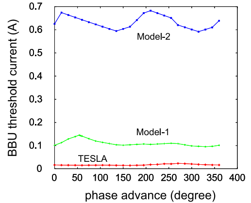
Figure 6: Threshold current for 3 types of cavities: TESLA, Model-1, Model-2.
