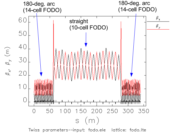
Figure 10: Betatron functions for the 1st loop.
