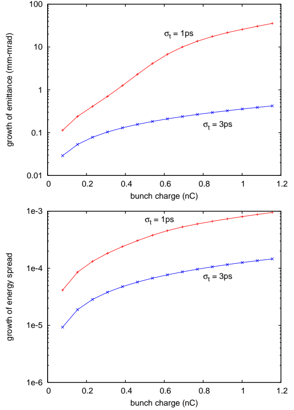
Figure 12: Growth of emittance and energy spread due to CSR effects in the 1st loop.
