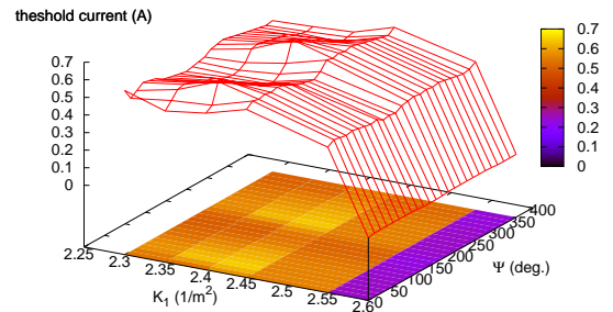
Figure 3: BBU threshold current for the 5 GeV ERL with Model-2 cavities as a function of beam optics, strength of the linac quadrupoles, K_1 , and phase advance of the return loop, \Psi .
