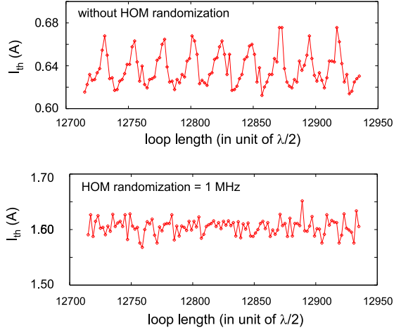
Figure 8: Threshold current against the variation of return-loop length.
