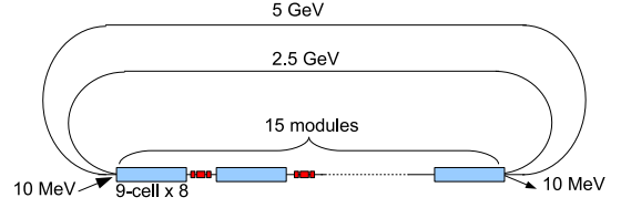
Figure 9: A 5 GeV ERL light source with a 2-turn configuration.
