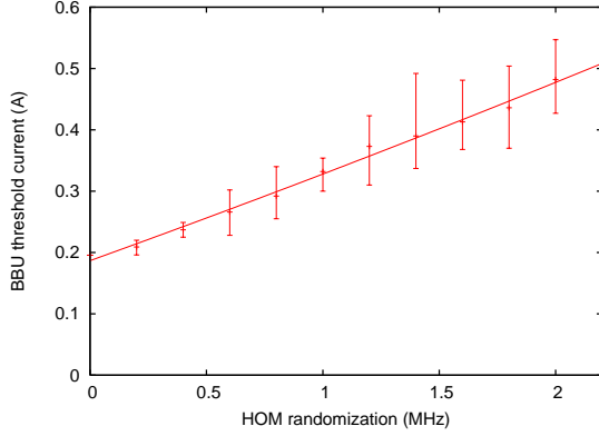
Figure 11: BBU threshold current of the 2-turn ERL with HOM frequency randomization.
