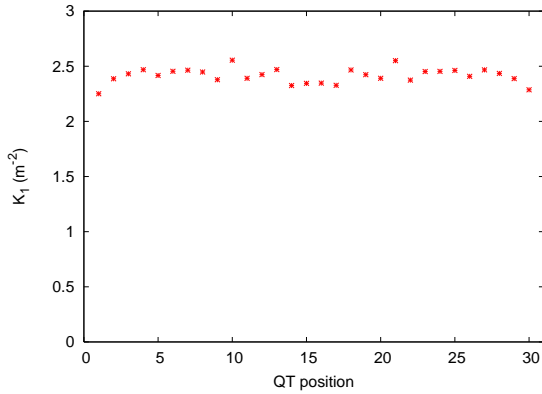
Figure 4: Optimum focusing strength of quadrupoles obtained from the “minimum beam size” scheme.
