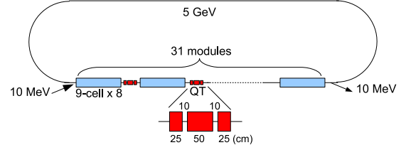
Figure 2: A 5 GeV ERL light source.
