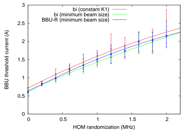
Figure 7: Threshold current with HOM frequency randomization for the 5 GeV ERL with Model-2 cavities.
