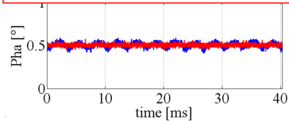
App. I: PS ripples rejection
