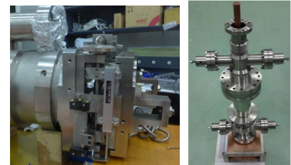
▼ Cavity tuners ready
