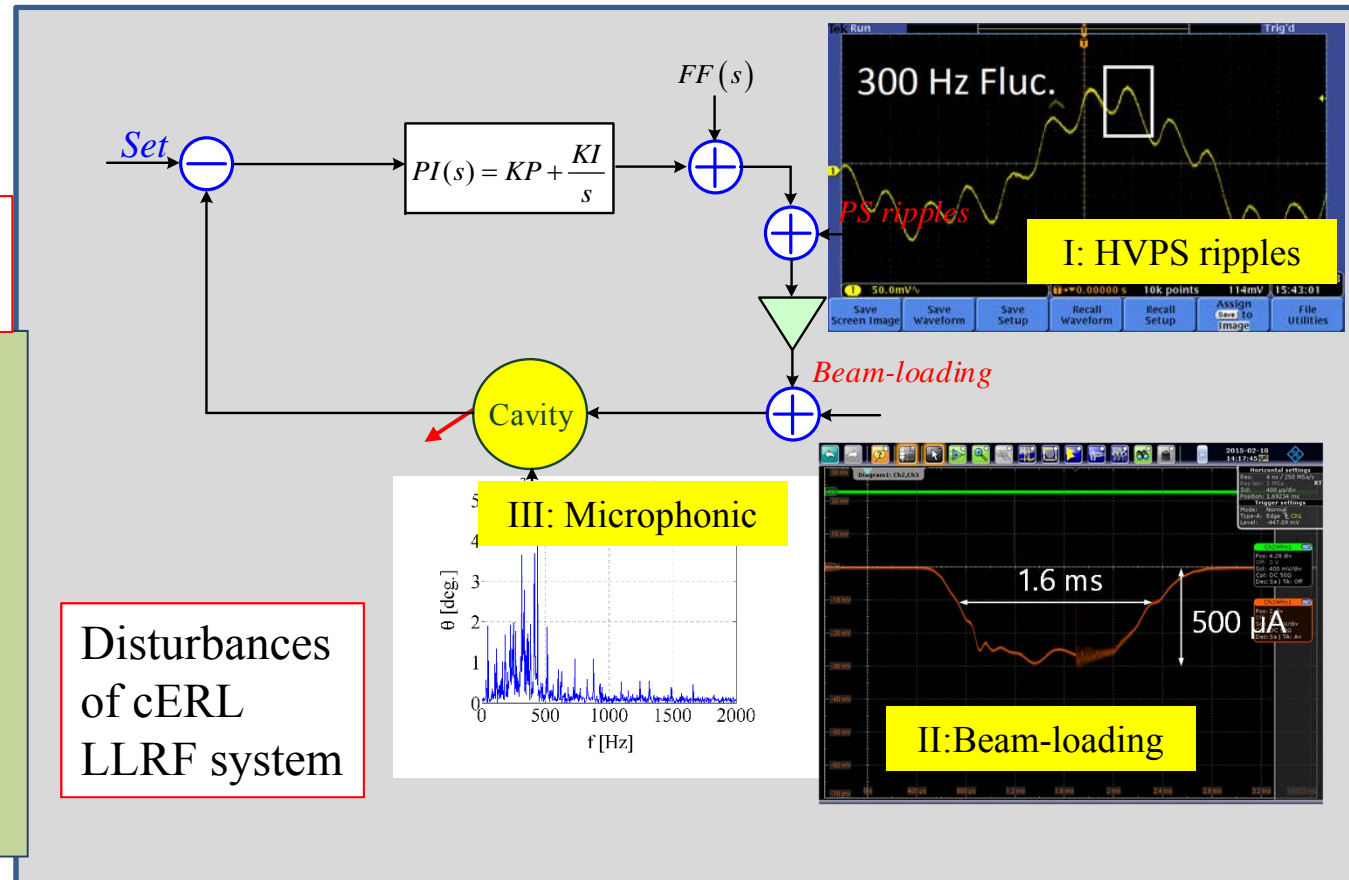
App. II: Beam-loading compensation
