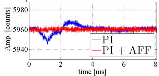
App. II: Beam-loading compensation
