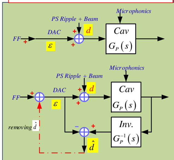
App. I: PS ripples rejection
